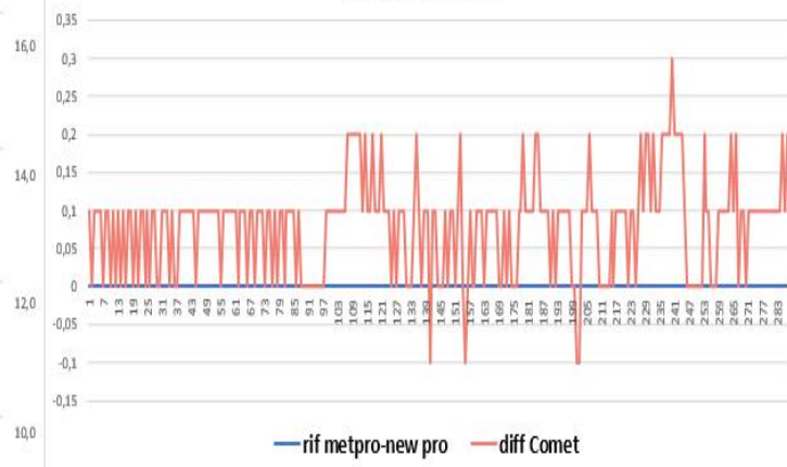
wind gust-solar
