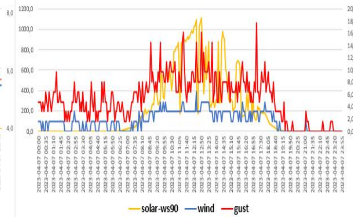
wind gust-solar
